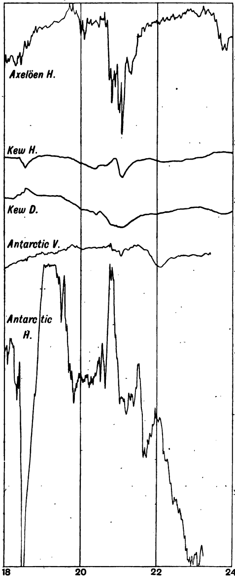
FIG. 25.—ARCTIC-KEW-ANTARCTIC CURVES.
